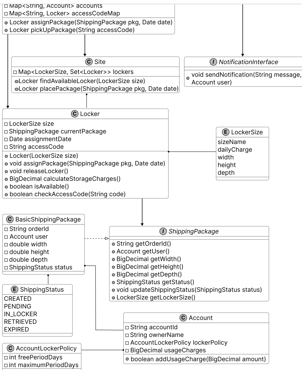
Class Diagram of Locker Service
